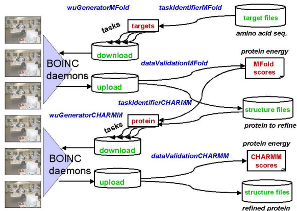
Figure 2. The P@H/BOINC structure.
